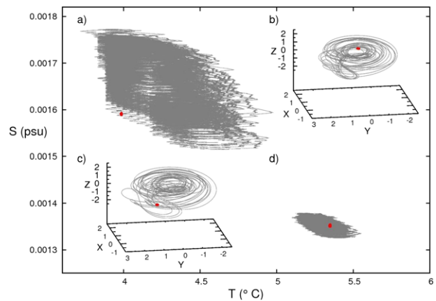
Figure 1. Trajectories of the L84-S61 model: ocean variables (latitudinal temperature ( T ) and salinity ( S ) differences) on the main axes, atmospheric variables ( X, Y, Z ) on insets. Ocean variables show 10 000 year simulations; atmospheric variables a single year. (a) and (b) show trajectories for F_m = 7 while (c) and (d) show trajectories for F_m = 8 . Red points show the IC locations of 10 000 member ensembles. For single ocean variable time series see supplementary figure S3 (available at stacks.iop.org/ERL/8/034021/mmedia ) ( F_m = 7 ) and figure S4 (available at stacks.iop.org/ERL/8/034021/mmedia ) ( F_m = 8 ).
