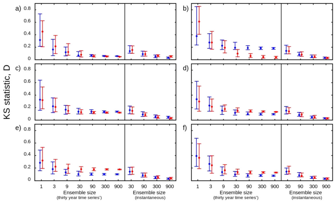
Figure 4. Comparisons of the ability of different methods and ensemble sizes to represent the model climate; each panel contains results from the variable and forcing scenario of the corresponding panel in figure 3. Plots show the KS statistic between a 10 000 member IC ensemble distribution constructed at 30 (blue) and 60 (red) years into a simulation with different methods of distribution construction. The right side of each subplot uses distributions constructed at the given time point (referred to as ‘instantaneous’ distributions), with varying ensemble size. The left side uses distributions constructed over a thirty year period around the given time point (‘kairoic’ distributions). Uncertainty is quantified by repeating the process 100 times using different ICs distributed around the same location on the attractor (see figure 1 and the supplementary materials available at stacks.iop.org/ERL/8/034021/mmedia ). Dots represent the median; errors are the 10th–90th percentiles.
