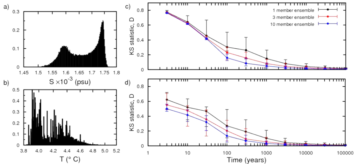
Figure 2. Convergence of distributions constructed from increasingly long trajectories, towards the long term distribution. (a) and (b) show normalized frequency distributions of S (a) and T (b) extracted from a single 100 000 year simulation. (c) and (d) show the difference, quantified by the KS statistic, between the (a) and (b) distributions and those generated using shorter simulations, for S (c) and T (d). The distributions are constructed from either single simulations (black) or by combining data up to the given time point from multiple simulations with different ICs; red—three simulations, blue—ten simulations. Uncertainty is quantified by repeating the process 100 times using different ICs distributed around the same location on the attractor (see figure 1 and the supplementary materials available at stacks.iop.org/ERL/8/034021/mmedia ); error bars do not therefore represent uncertainty in our assessment of D but rather the distribution of values from which any particular simulation/ensemble may be considered a draw. Lines connect the median values at each time point; errors are the 10th–90th percentiles.
