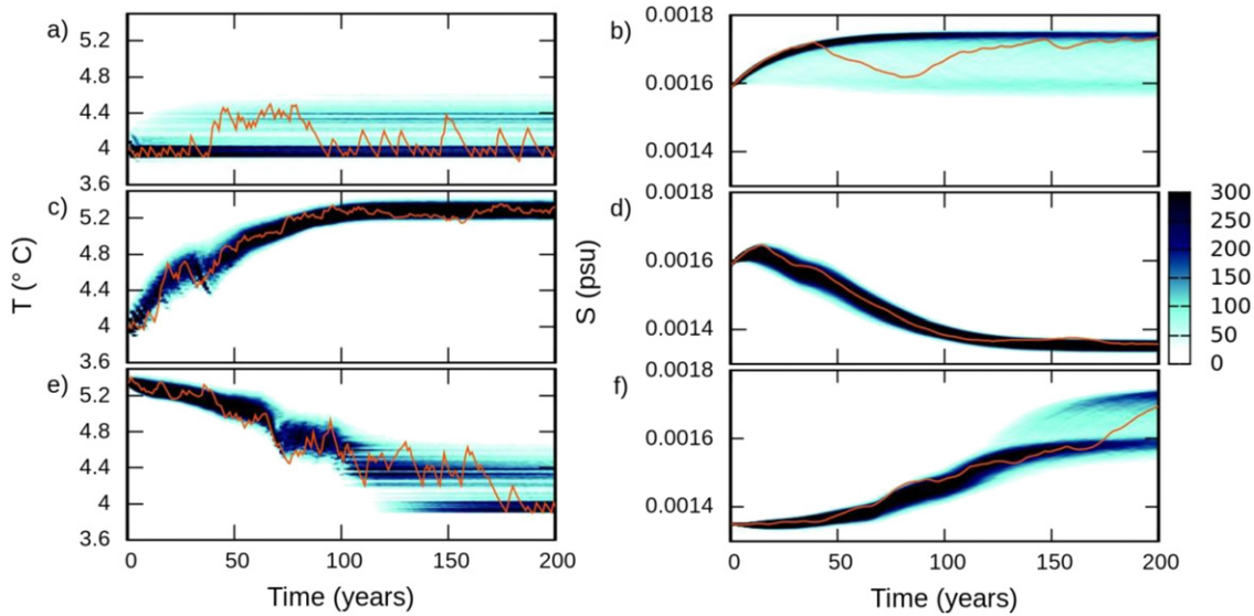
Figure 3. Time-dependent probability density functions for T and S from 10 000 member ensembles. ICs are centred on the locations on the attractor shown in figure 1 (see construction method in the supplementary materials available at stacks.iop.org/ERL/8/034021/mmedia ). F_m varies as follows: (a) and (b) F_m = 7 ; (c) and (d) F_m increases linearly from 7 to 8 over 100 years and is then fixed at F_m = 8 ; (e) and (f) F_m decreases linearly from 8 to 7 over 100 years and is then fixed at F_m = 7 . The legend shows the frequency of ensemble members per 0.01^\circ\text{C} ( T ), per 2.5 \times 10^{-6} psu ( S ). Single trajectories originating from the central state of the IC ensembles are shown in orange.
